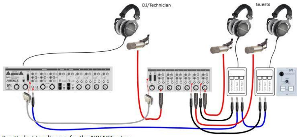
Practical wiring diagram for the AIRENCE mixer
