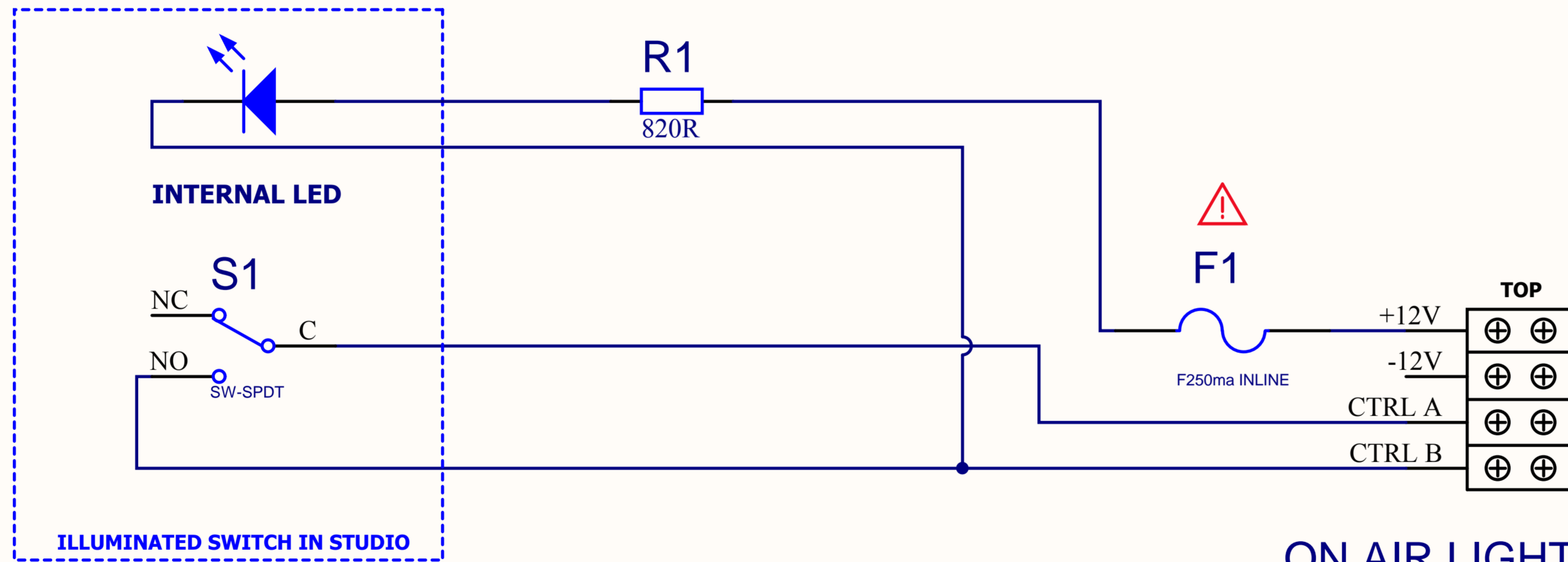
ON AIR LIGHT TERMINALS
